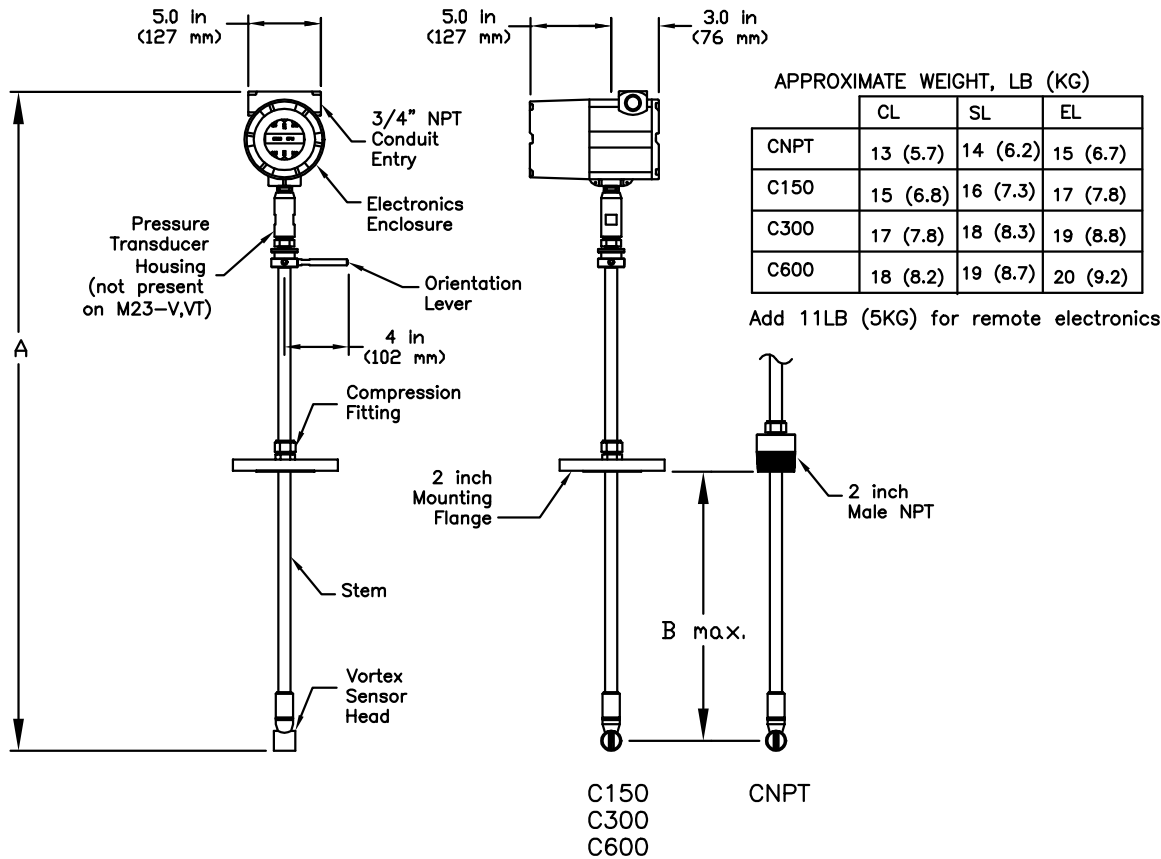
MODEL M23-V,VT in (mm)
