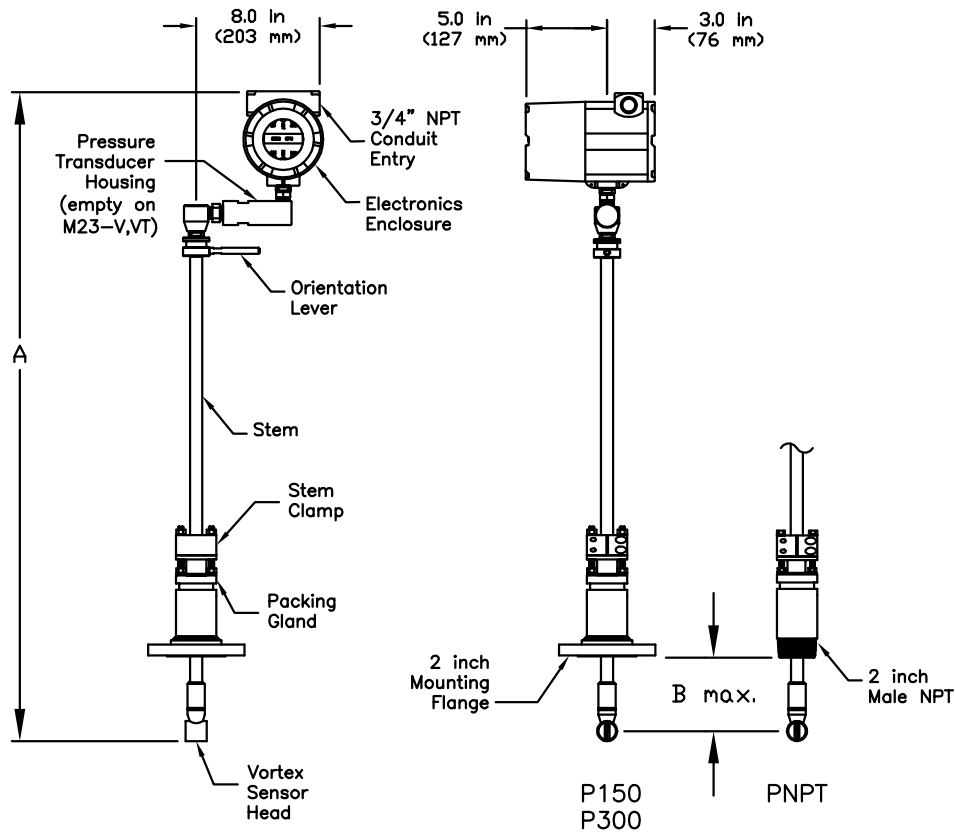
MODEL M23 in (mm)
